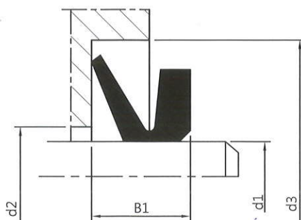
Dimension table -V-Ring Type VL
